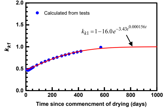
Fig. 6 Drying shrinkage factor on k_I ( k_{kI} )
