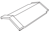
Vee Ridge (130°) Dimensions: 435L x 265W x 88D Cover length: 400
