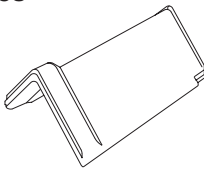
Steep Pitch Vee Ridge (81°) For roofs over 45° in pitch Dimensions: 435L x 265W x 185D Cover length: 400
