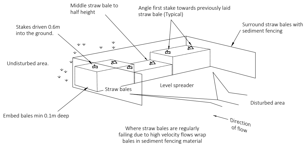
Drainage Discharge Point
