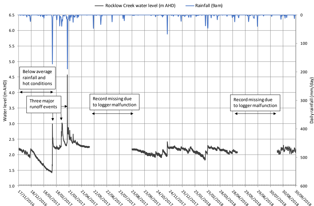
Figure 3.3 Water level data – Rocklow Creek
