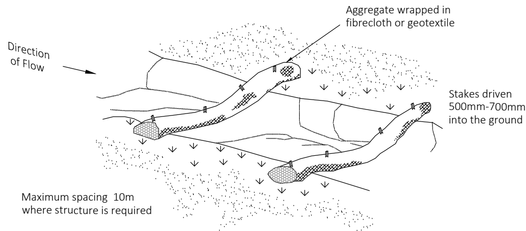
Filter Sock
