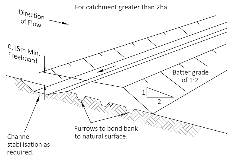
Diversion Bank and Channel
