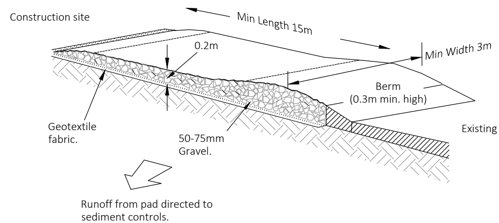
Temporary Construction Entry / Exit
