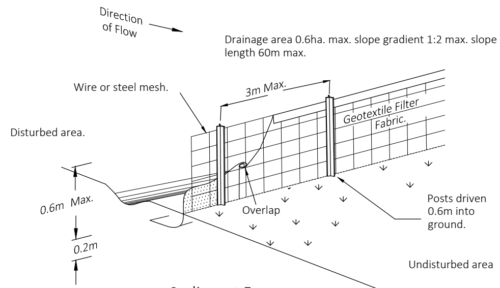
Sediment Fence
